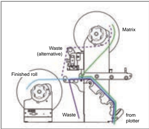
MATRIX REMOVER AND SLITTER MODULE
